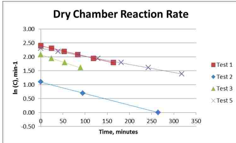
Figure 41 Dry Chamber Reaction Rate
